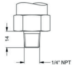
1/4" -18NPT
